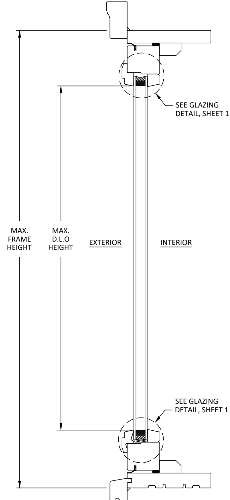
B 4 VERTICAL SECTION 4-9/16" FRAME ARCHTOP
