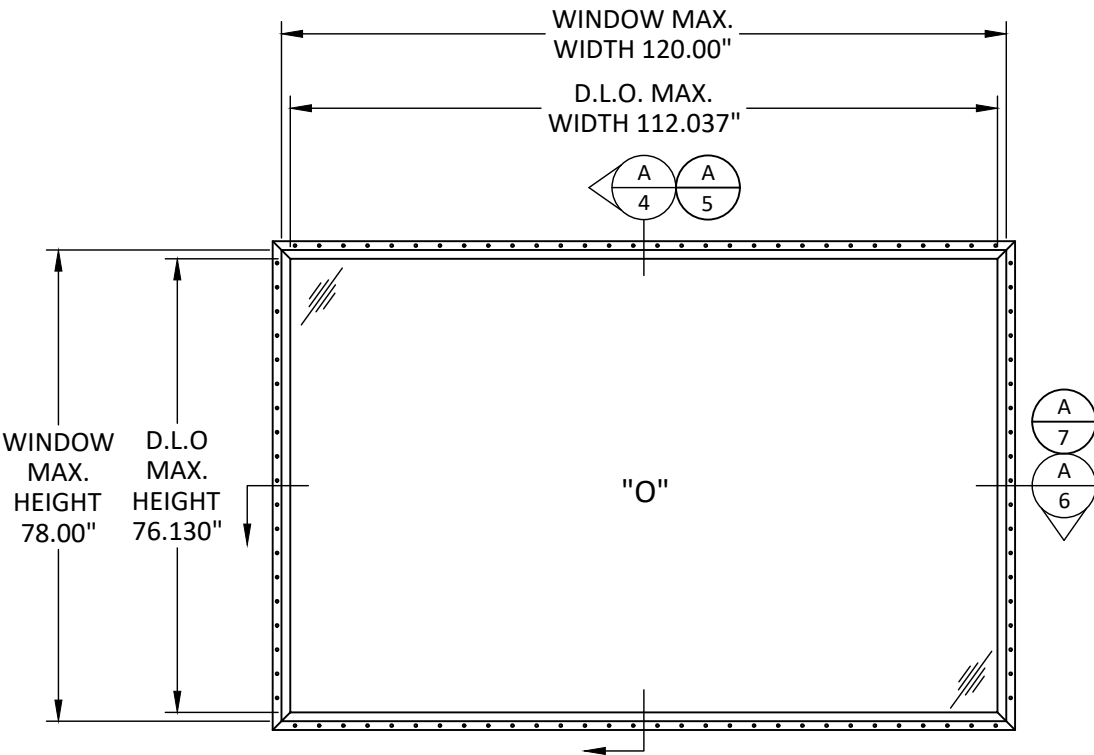
ELEVATION RECTANGULAR
