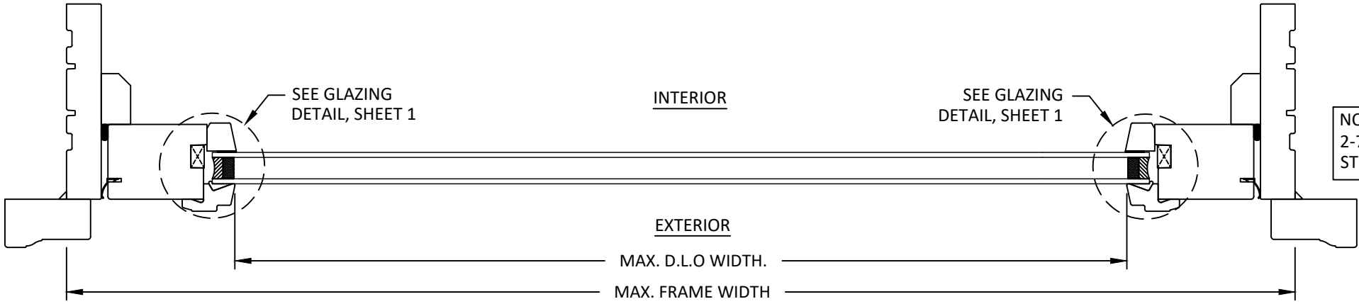
B 6 HORIZONTAL SECTION 4-9/16" FRAME ARCHTOP
