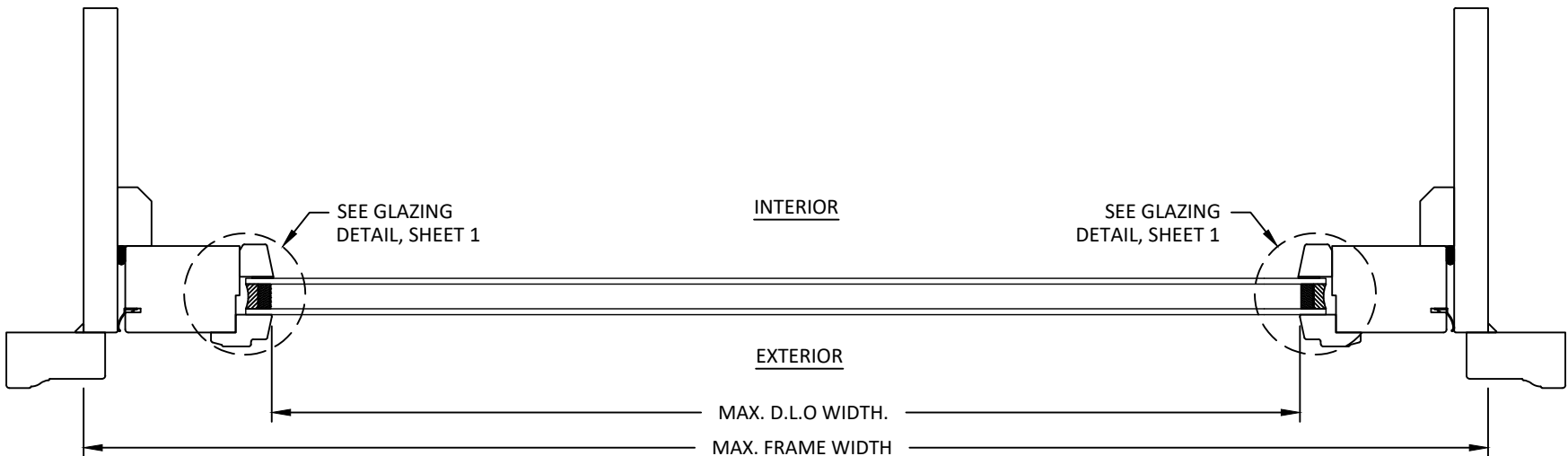
C 7 HORIZONTAL SECTION 6-9/16" FRAME SPRINGLINE
