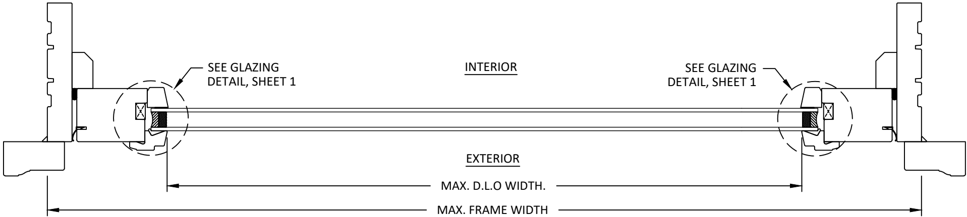
A 6 HORIZONTAL SECTION 4-9/16" FRAME RECTANGULAR
