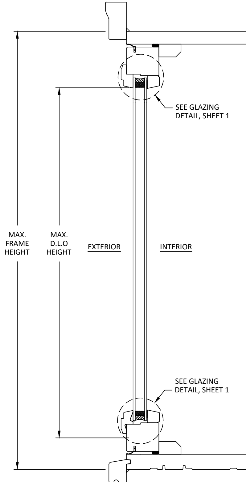
B 5 VERTICAL SECTION 6-9/16" FRAME ARCHTOP
