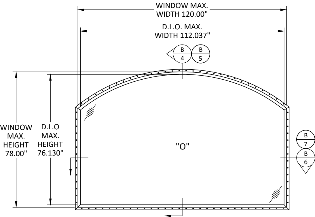
ELEVATION ARCHTOP
