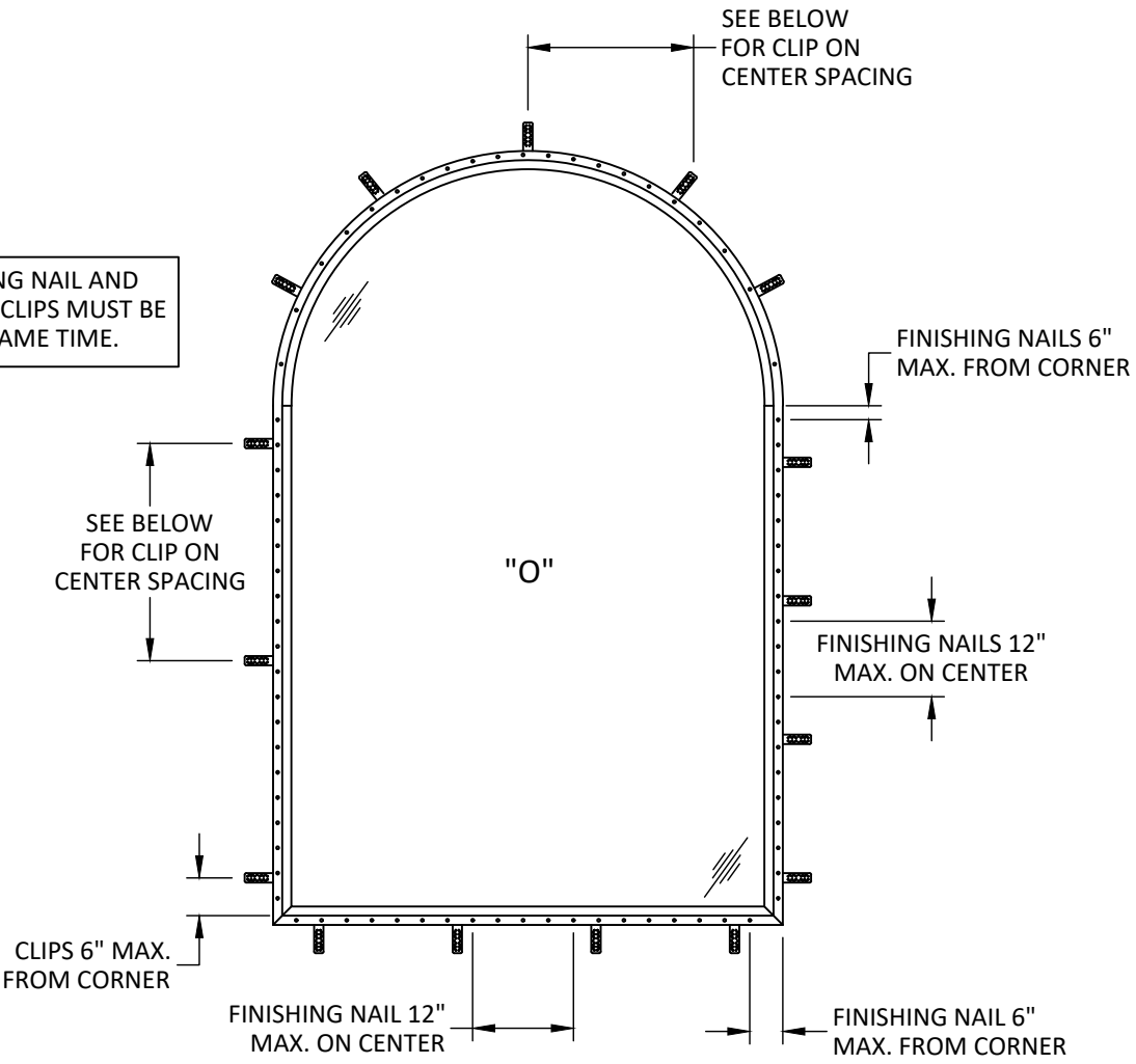
ANCHOR LAYOUT SPRINGLINE
