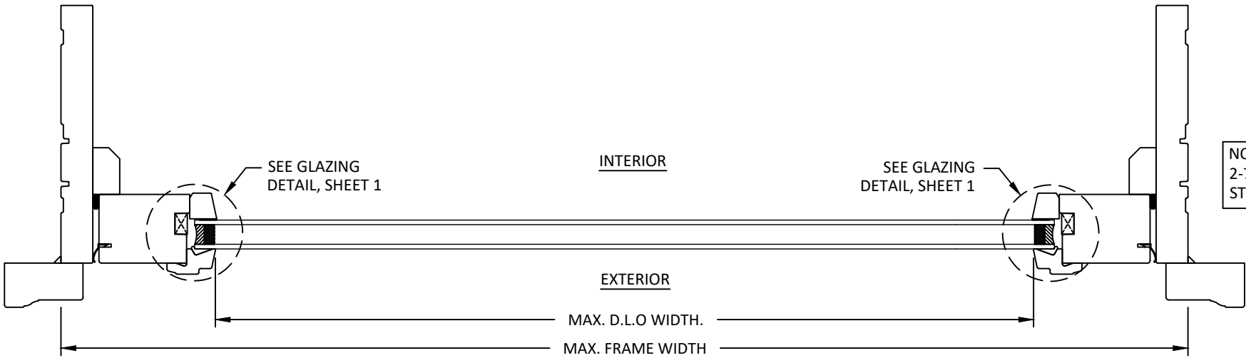
B 7 HORIZONTAL SECTION 6-9/16" FRAME ARCHTOP
