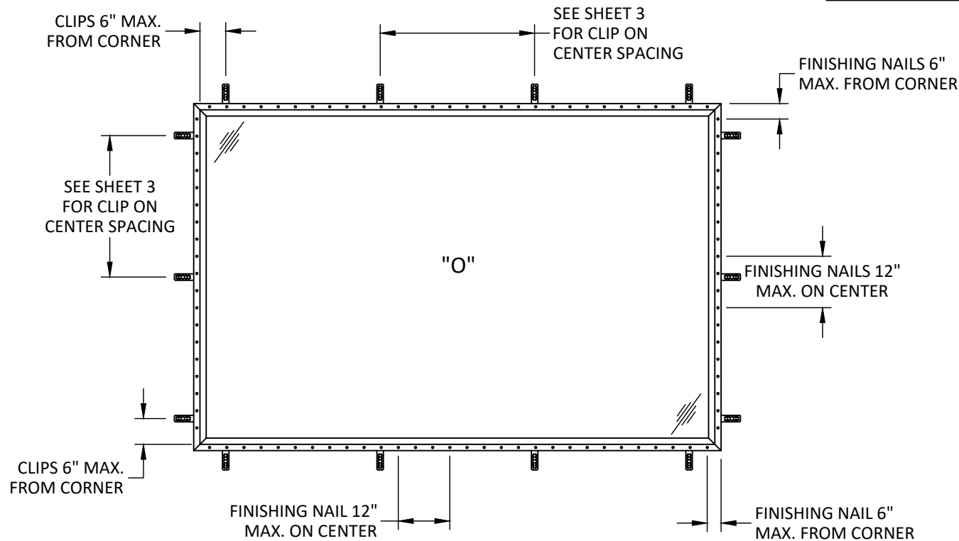
ANCHOR LAYOUT RECTANGULAR
