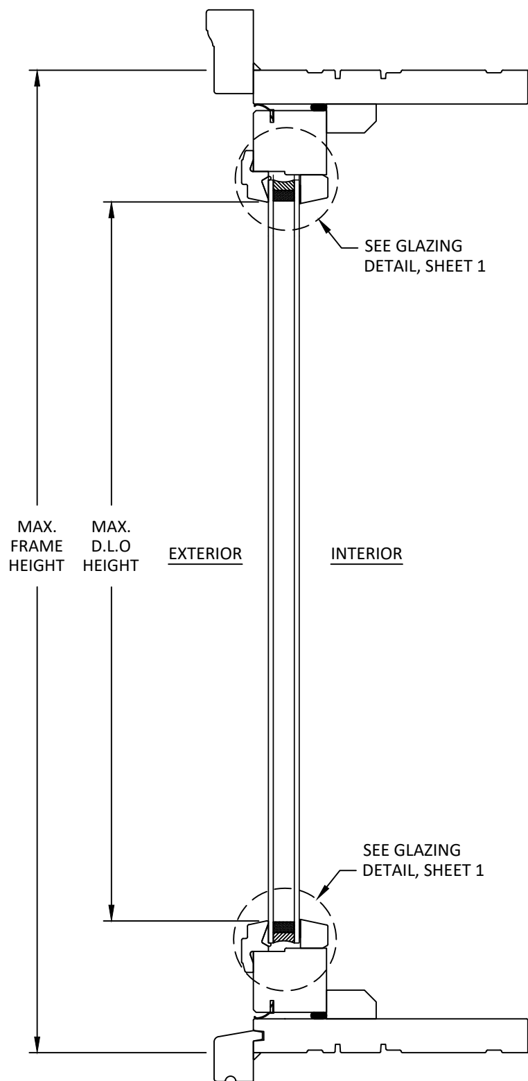
A 5 VERTICAL SECTION 6-9/16" FRAME RECTANGULAR
