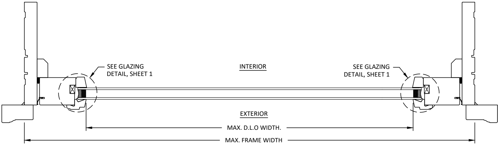
A 7 HORIZONTAL SECTION 6-9/16" FRAME RECTANGULAR
