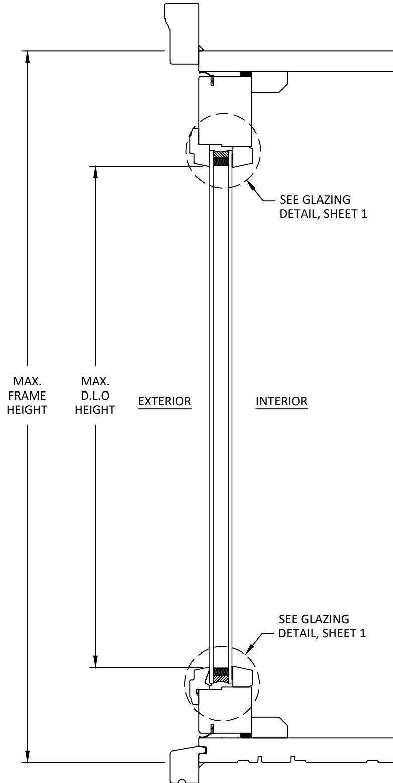
C 5 VERTICAL SECTION 6-9/16" FRAME SPRINGLINE
