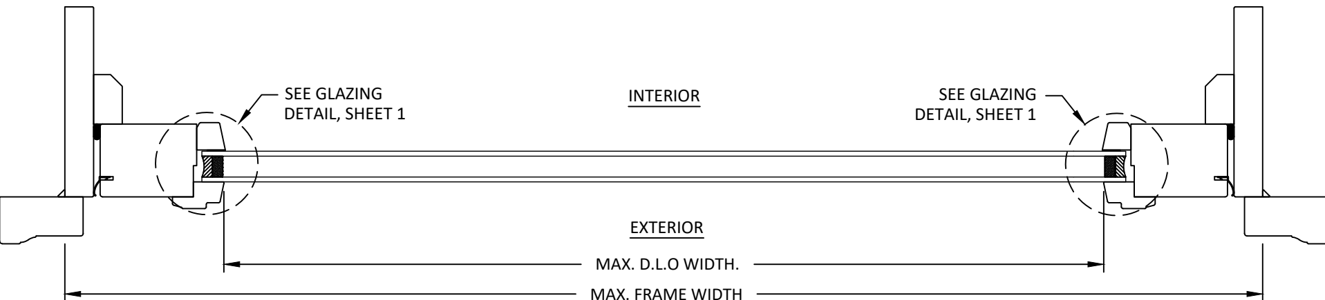
C 6 HORIZONTAL SECTION 4-9/16" FRAME SPRINGLINE
