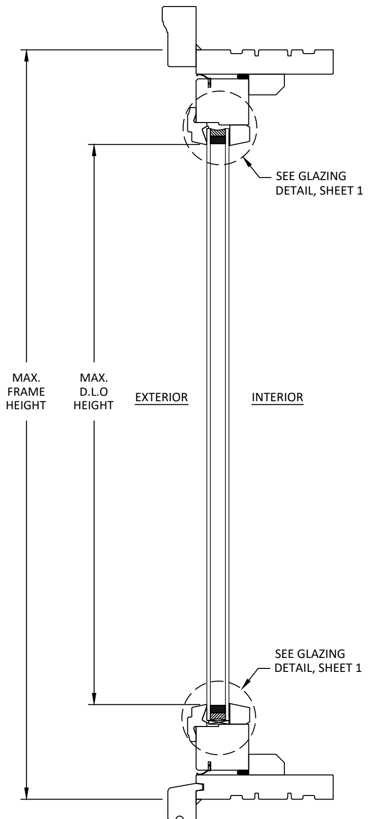
A 4 VERTICAL SECTION 4-9/16" FRAME RECTANGULAR
