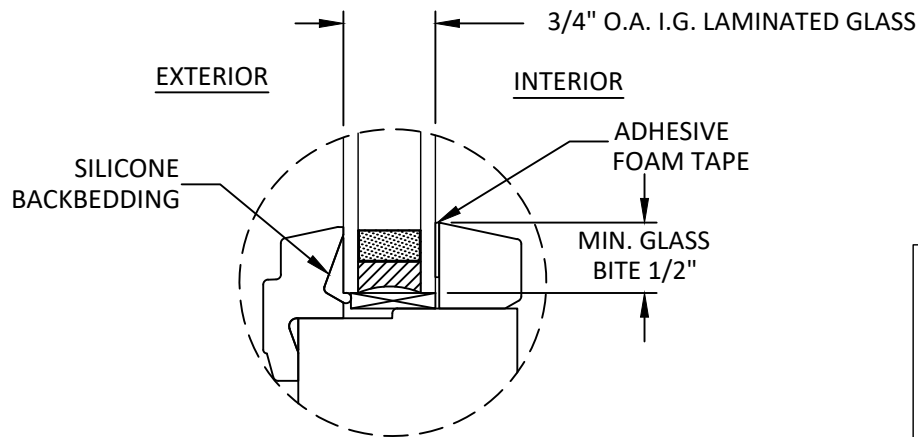
GLAZING DETAIL 1
