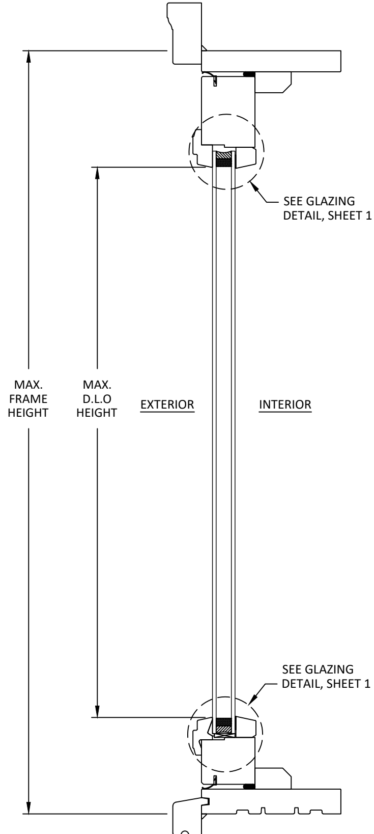
C 4 VERTICAL SECTION 4-9/16" FRAME SPRINGLINE
