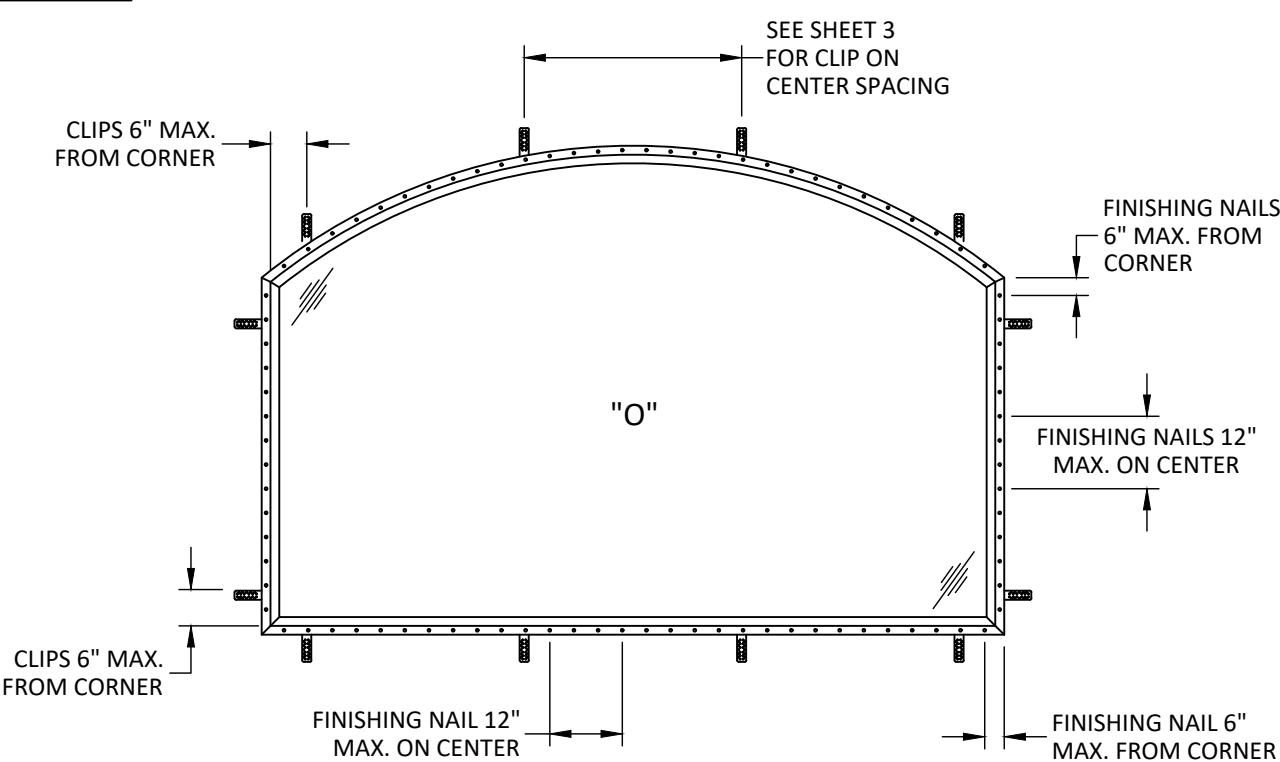
ANCHOR LAYOUT ARCHTOP
